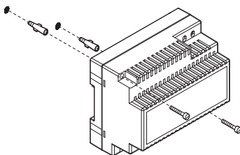
Wall-mounted installation
